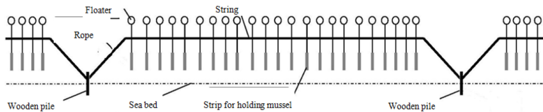
Fig. 2 is the depiction of farms engaged in mussel cultivation
